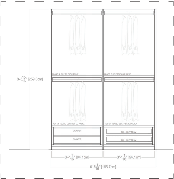
OCEAN WARDROBE - ELEVATION (OPEN DOORS)
